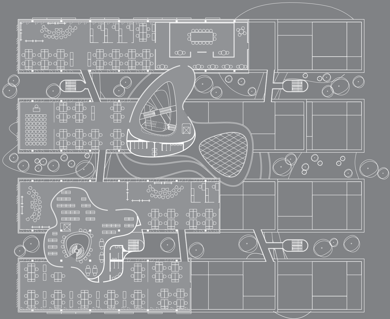
fourth floor 1/250
