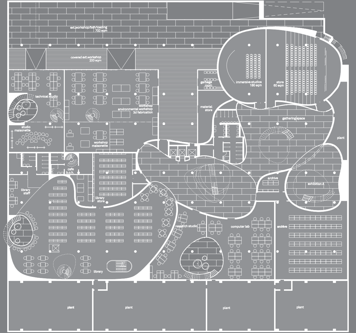
lower ground floor 1/500
